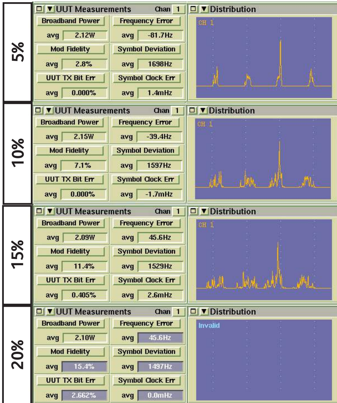
Figure 14: P25 Deviation Balance Negative Calibration Errors
