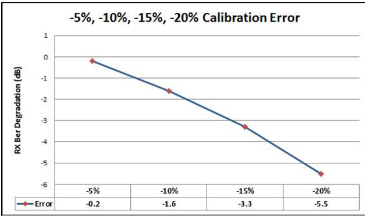
Figure 18: P25 RX BER Degradation Due to Deviation Balance Misalignment (NEG)
